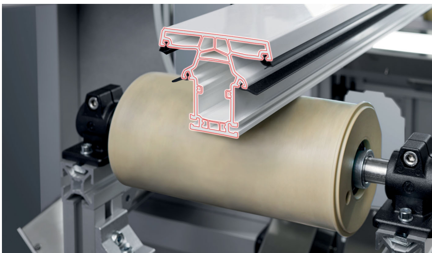
Pixargus inspects the inner cross section and the clamping sections of cut plastic or metal profiles in extrusion lines directly after the cutting device and, as a first, also measures the rates of recycled materials in the process. (Source: PIXARGUS)
