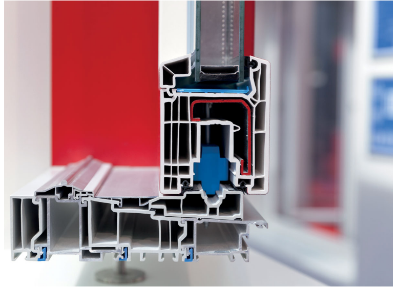
Today's high-grade recycled plastics are suitable materials for use in the cores of high-tech profiles. (Source: iStock)
