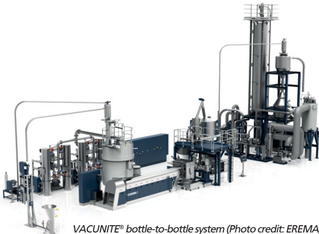
VACUNITE® bottle-to-bottle system (Photo credit: EREMA)
