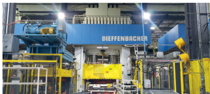
DIEFFENBACHER hydraulic press at CSP's Sarepta, Louisiana, site
