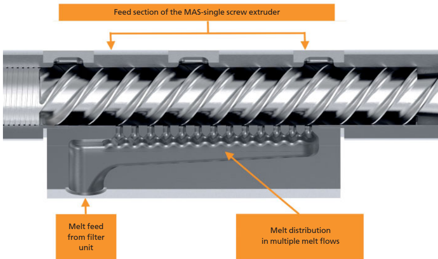
Picture 7: Section through the "multi-channel melt feed block", in which the melt flow coming from the melt filter is divided into individual melt flows (Picture: MAS)
