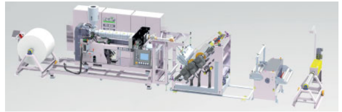
MEAF Machines has added a PROMIX physical foaming installation to its in-house extruder test and demonstration line. As of mid-May this will allow customers to get hands-on experience with this material saving equipment while using their own polymer grades in the process (Source: MEAF)
