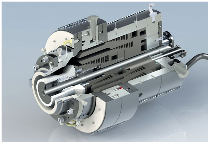
Four layers pipe-head
