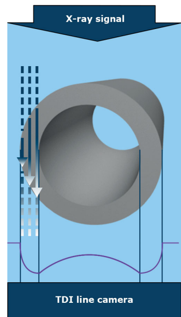
Picture 1: Design and functional principle of the measurement with X-ray technology
